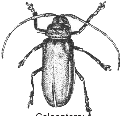
Coleoptera: beetles
