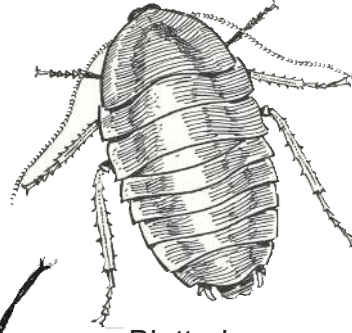
Blattodea: cockroaches
